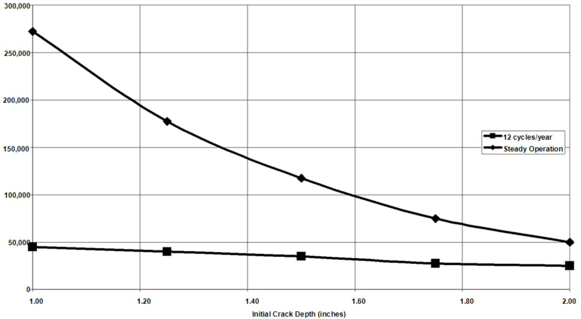
Figure 2 - Impact of Cycling on Useful Life of Header
